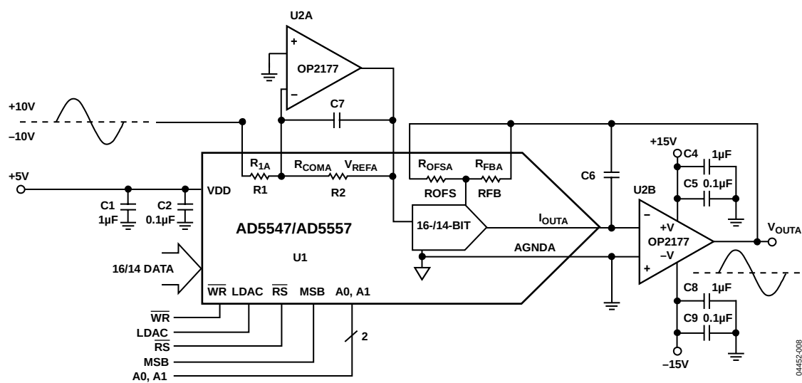
Figure 24. Signal Attenuator with AC Reference
